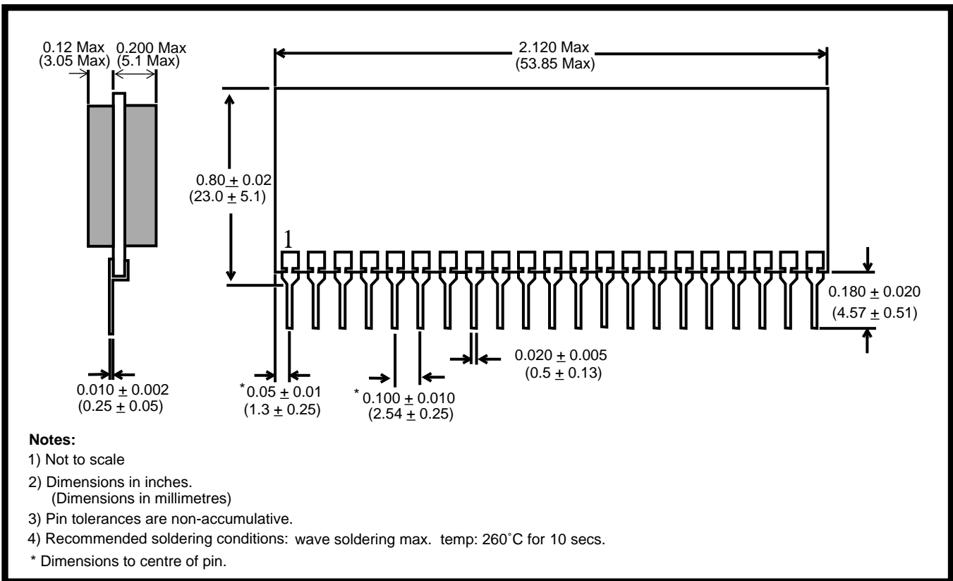
Figure 11 - Mechanical Data for 21 Pin SIL Hybrid
