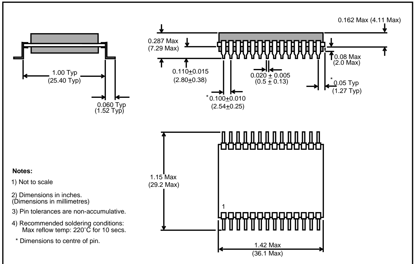
Figure 13 - Mechanical Data for 28 Pin SMT
