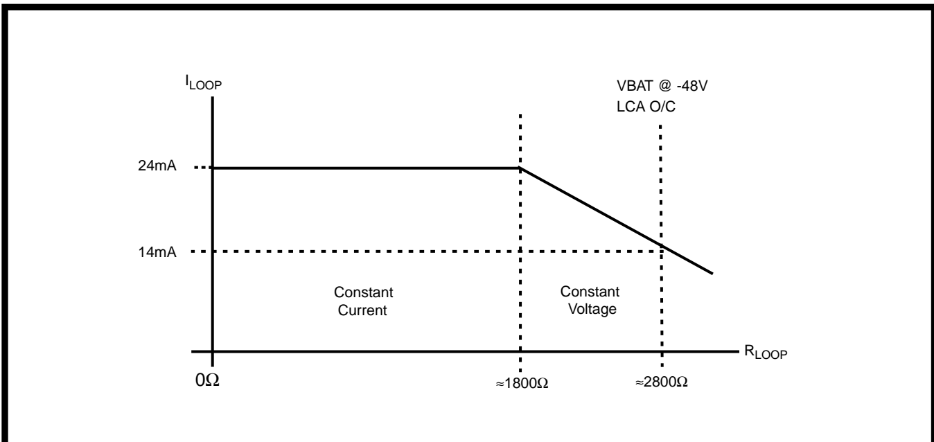
Figure 4 - Loop Current v Line Resistance
