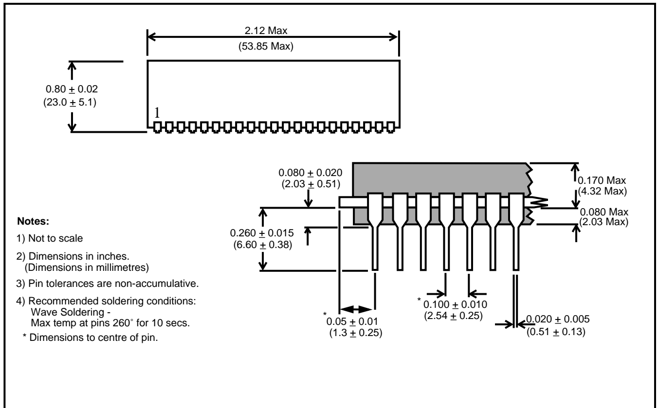
Figure 14 - Mechanical Data for 28 Pin T Bend
