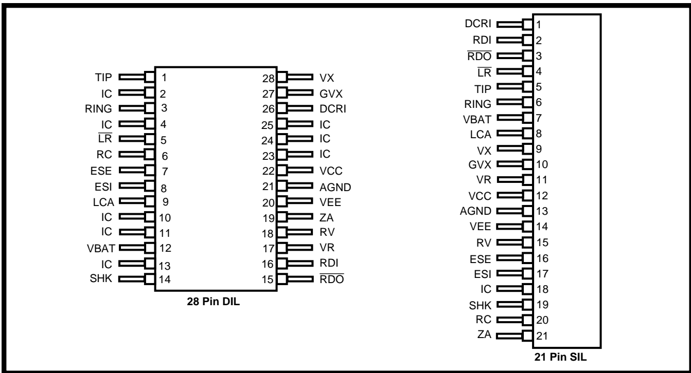
Figure 2 - Pin Connections
